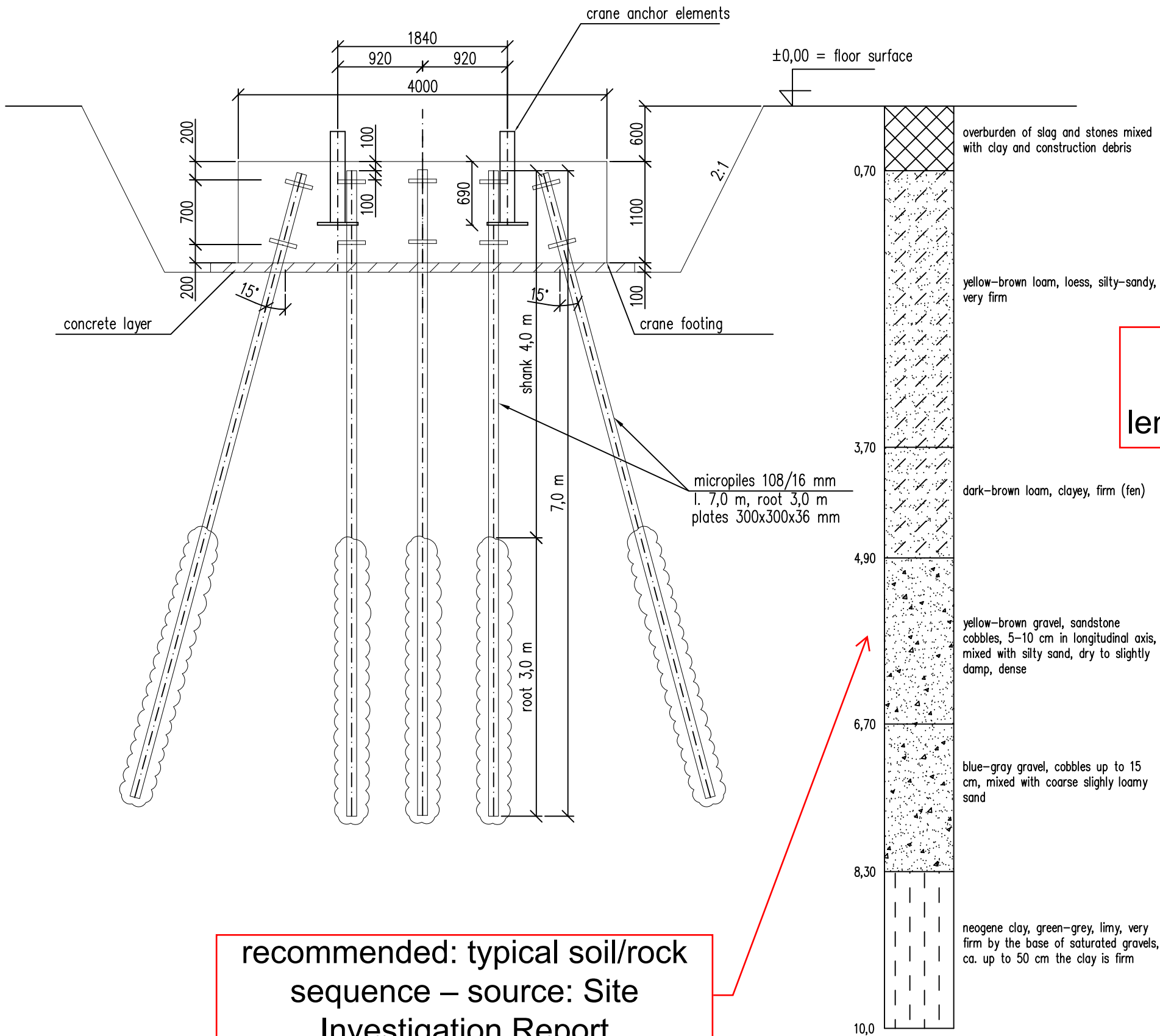
Section with dimensions and specification of micropiles and their fixing in the square pad footing)
