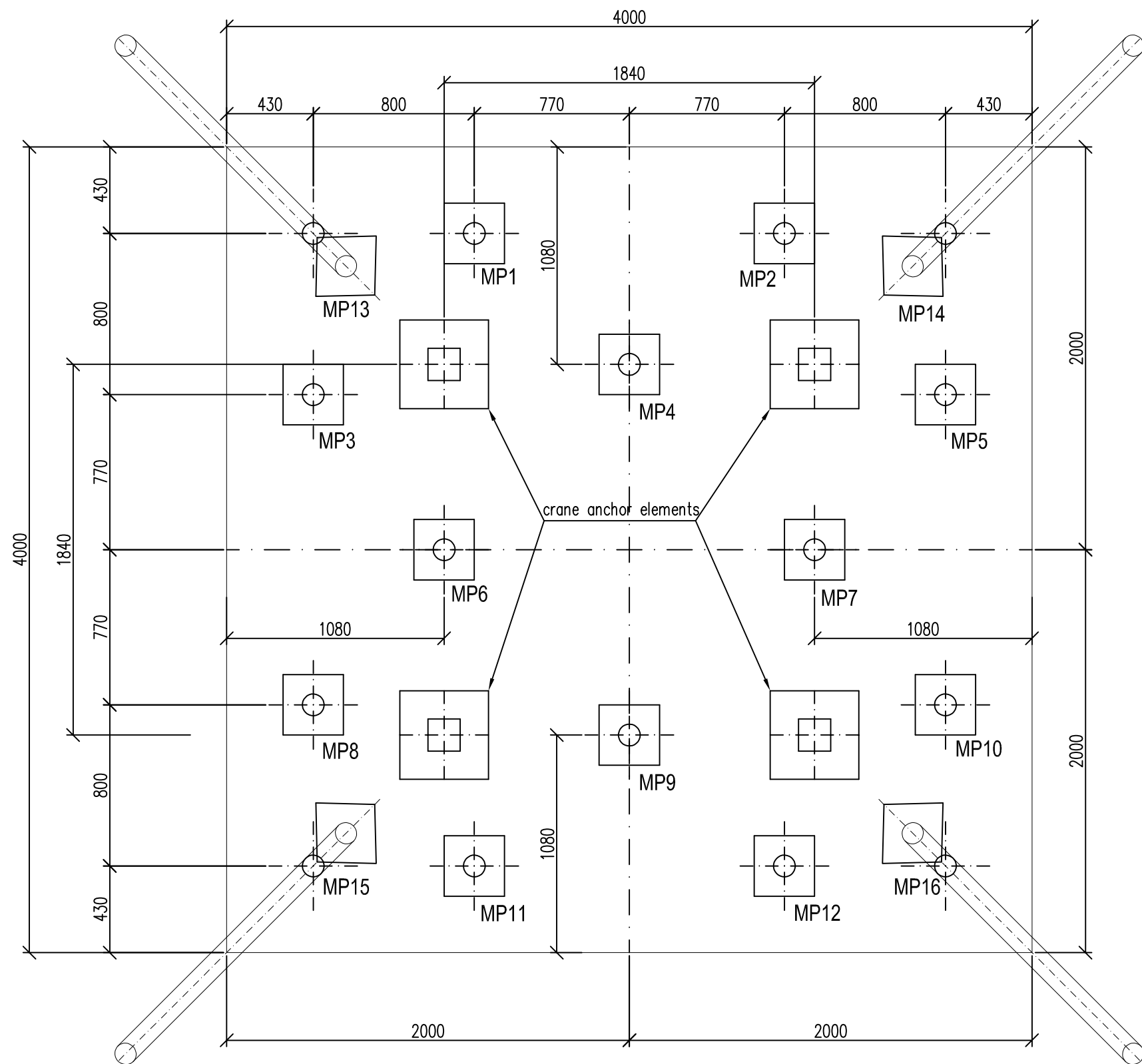
Plan view with dimensions and micropiles indication
